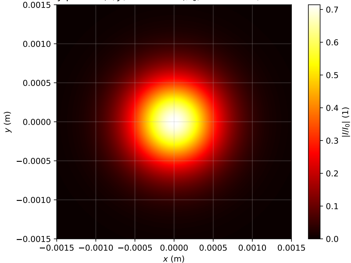
Intensity profile I(x, y, z = 2.388m)/I_0 , P_{in}=0.5P_{cr} , artificial time
